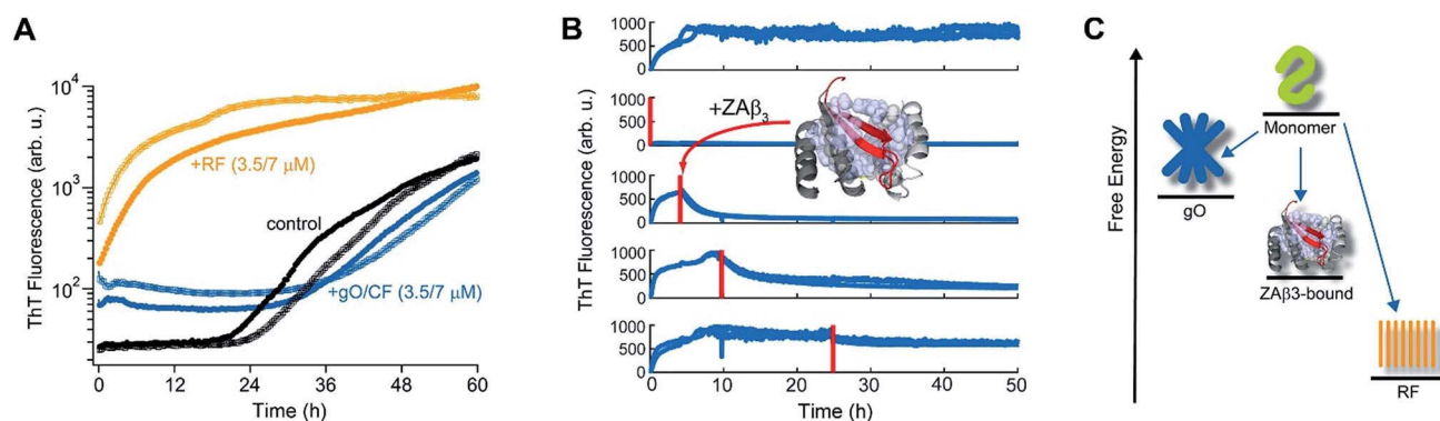
Fig. 3 Metastability and RF seeding incompetence of gO/CFs. (A) HewL RF kinetics below the COC (38 \mu M hewL, 400 mM NaCl) without seeding (black), or after seeding with isolated gO/CFs (blue) or RFs (orange) at either 3.5 or 7 \mu M each, and incubated at pH 2, T = 52^\circ\text{C} . (B) ThT-detected dissociation of pre-assembled dimA \beta upon addition of the binding protein ZA \beta 3 (grey), which sequesters monomeric dimA \beta in a \beta -hairpin conformation (red, see ref. 65 and 67). The complex is shown in ribbon representation, hydrophobic side chains of ZA \beta 3 in direct contact with the A \beta 40 \beta -hairpin are shown as spheres (Protein Data Bank entry 2OTK). The assembly of 6 \mu M dimA \beta was monitored by ThT fluorescence, with addition of 14 \mu M ZA \beta 3 at different time points, indicated by red lines. Addition of ZA \beta 3 during the gO/CF formation-dominated time regime results in nearly complete loss of ThT fluorescence, while ZA \beta 3 addition during the RF-dominated time regime leads to a progressive decrease in the amplitude of the fluorescence drop. (C) Energy diagram illustrating the order of thermodynamic stability of different states of A \beta , above the COC and under the present experimental conditions.
